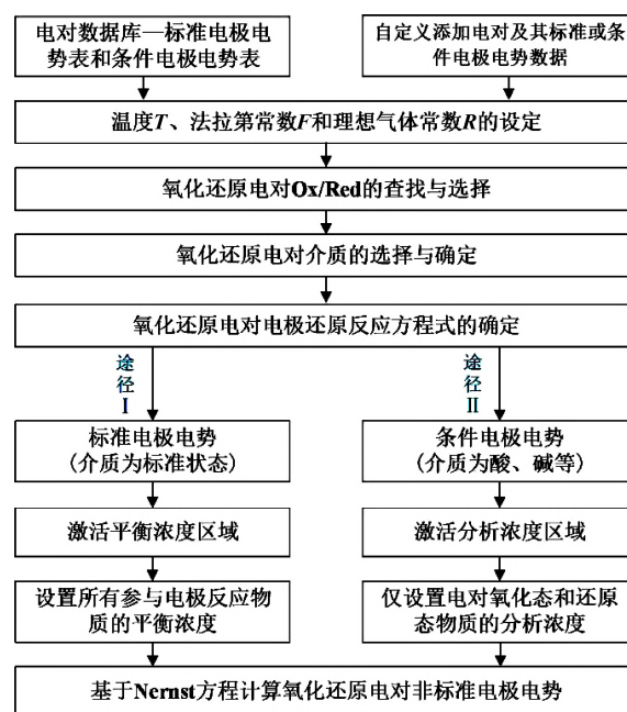
Fig. 2 The two routes for calculation of electrode potential in non-standard state
